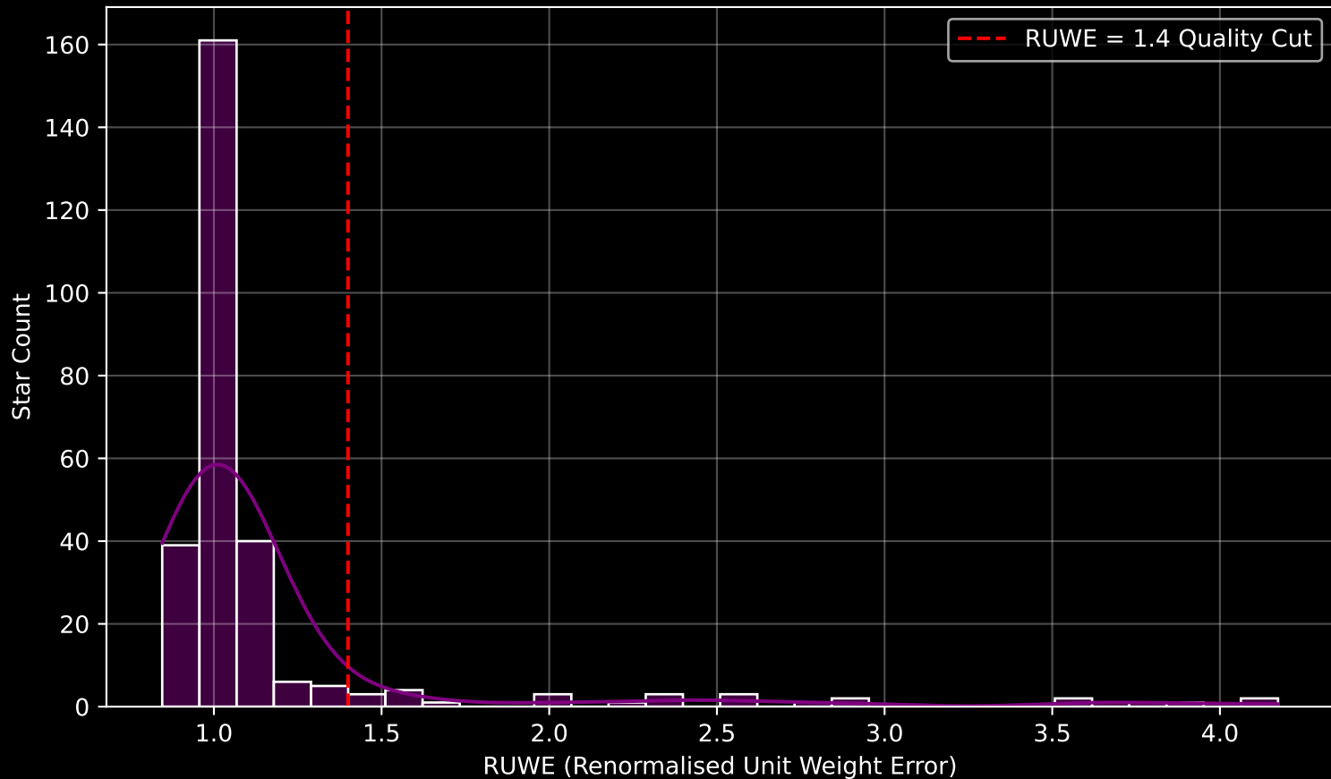
GALAH DR4 Field [6997] RUWE Distribution (n= 279)
