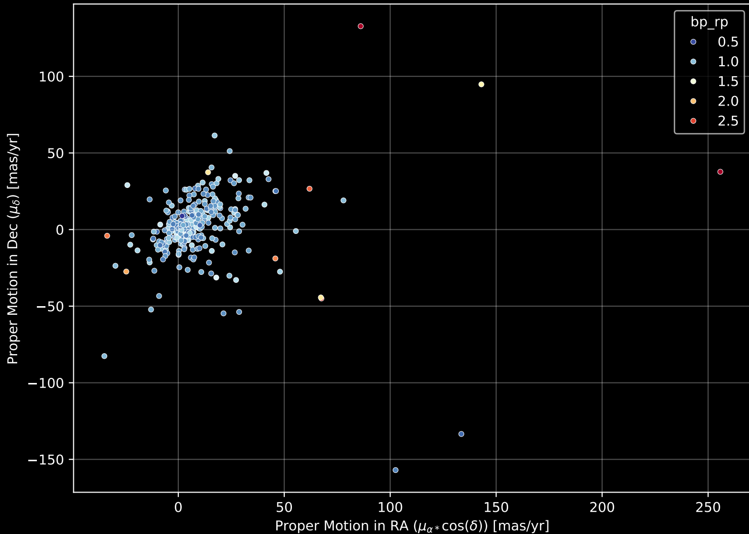
GALAH DR4 Field: [6997] Proper Motion Diagram (n= 288)
