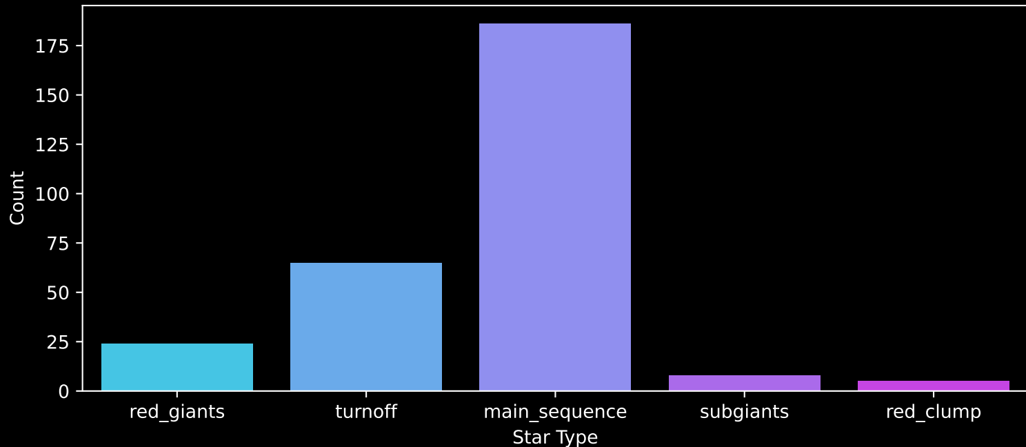
GALAH DR4 Field: [6997] Count plot of Star Type
