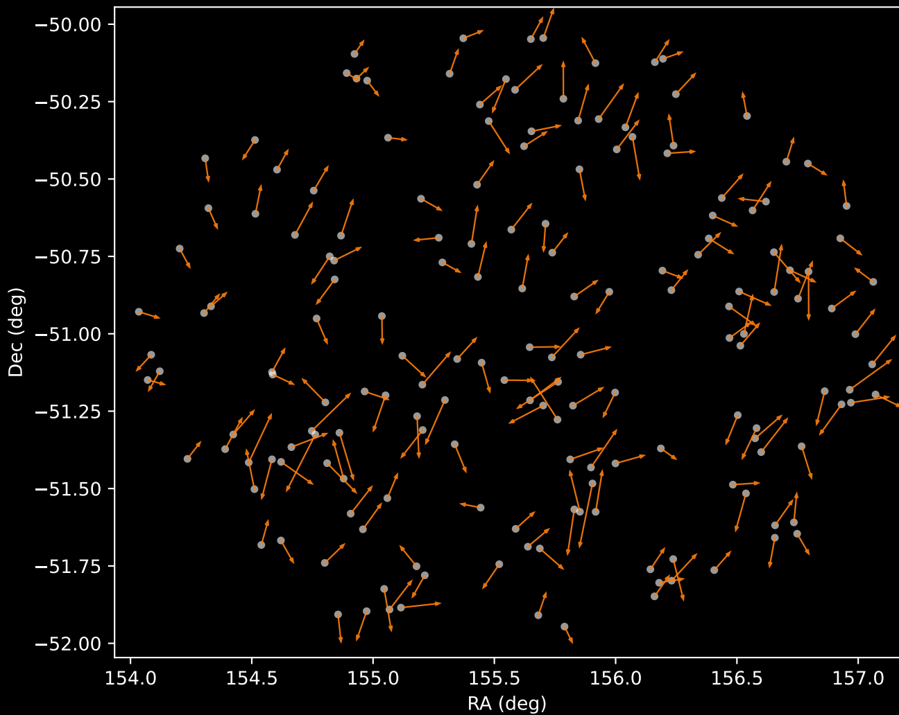
GALAH DR4 Cluster 2 Proper Motion Vectors (n=173)
